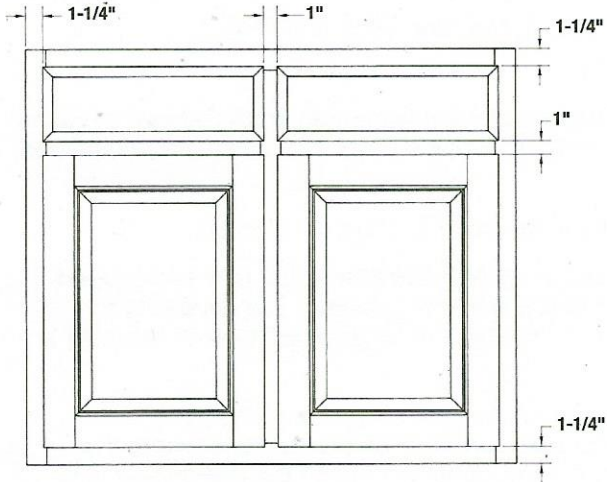
1-1/4" Overlay
