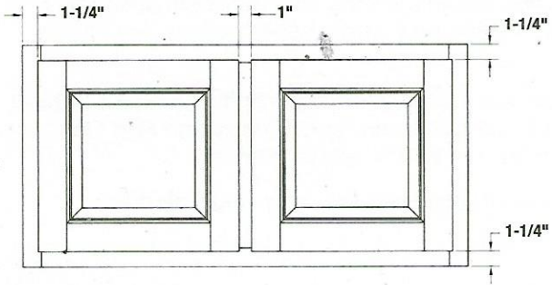
1/4" Overlay
