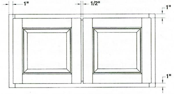
1/2" Overlay
